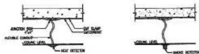
HEAT & SMOKE DETECTOR INSTALLATION DETAIL
