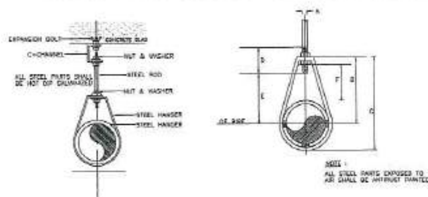
PIPE HANGER SIZE UP TO 50mm (2"φ)
