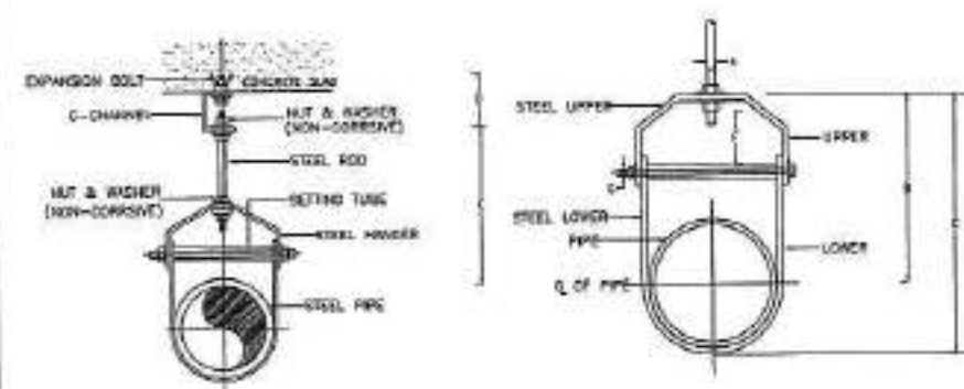
PIPE HANGER SIZE 65mm (2 1/2") AND LARGER
