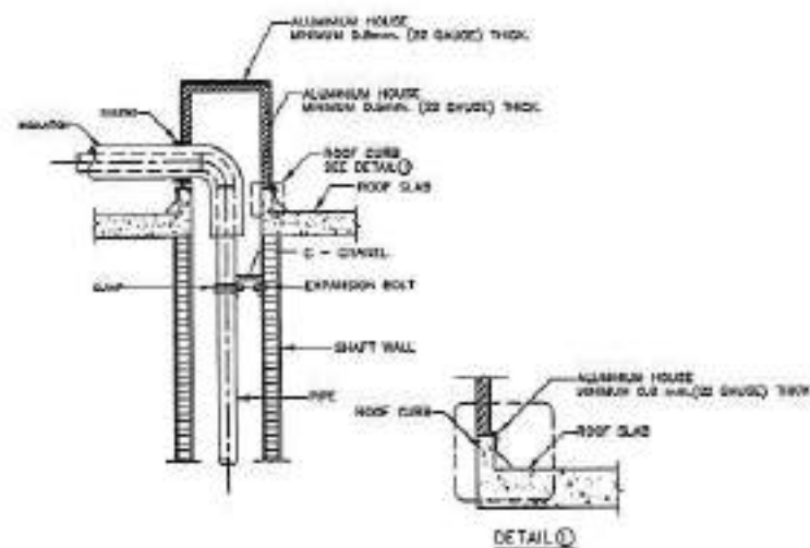
PIPE THRU ROOF RAIN PROJECTION
