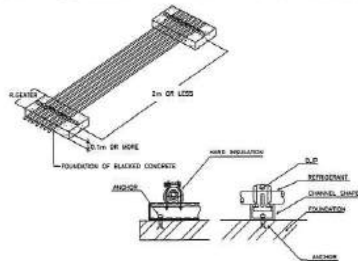
HORIZONTAL REFRIGERANT PIPES SUPPORT
