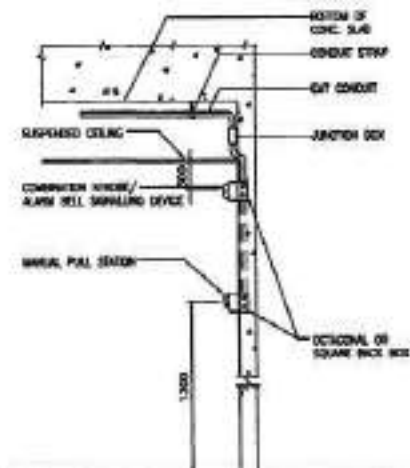
MANUAL PULL STATION, STROBE AND ALARM BELL INSTALLATION
