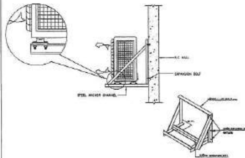
HORIZONTAL DISCHARGE CONDENSING UNIT WALL MOUNTING DETAIL
