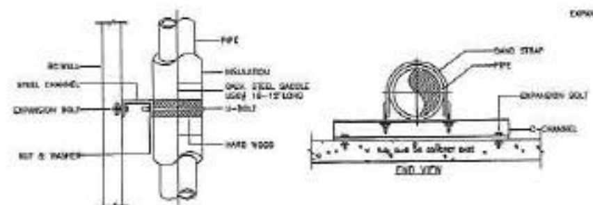
PIPE GUIDE (STRAP TYPE)
