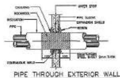
PIPE THROUGH EXTERIOR WALL
