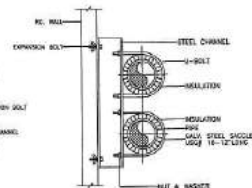
INSULATED PIPE SUPPORT TO WALL
