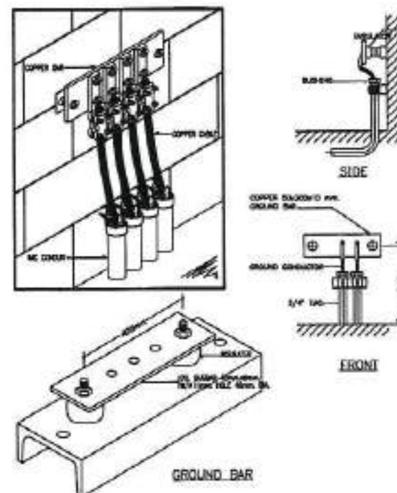
GROUND BAR INSTALLATION
