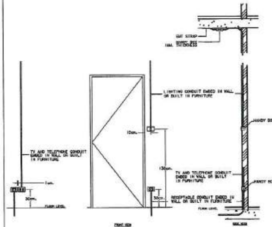
RECEPTACLE & TV/TELEPHONE OUTLET INSTALLATION
