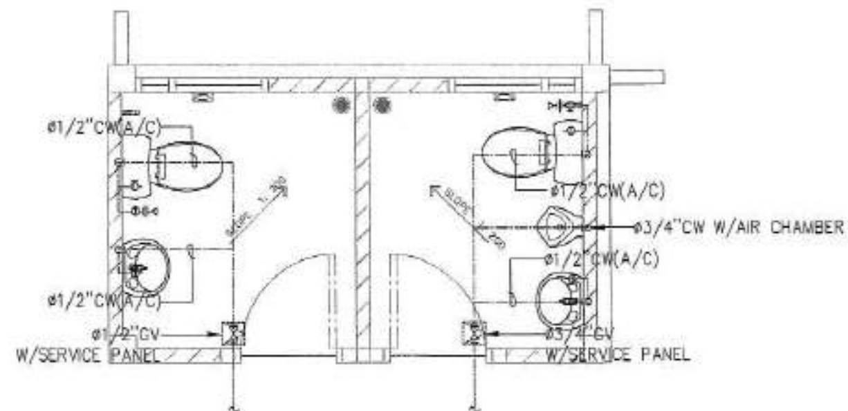
DETAIL COLD WATER FOR TOILET
